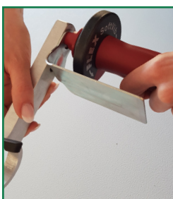
Mount the protective plate to the holder with the screw of the angle grinder handle
